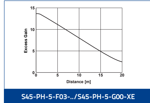
EXCESS GAIN
