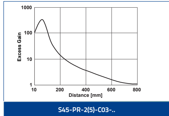
EXCESS GAIN
