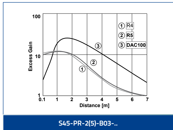
EXCESS GAIN
