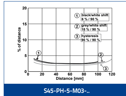
B/W SHIFT
